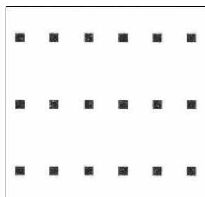
Pattern 8 Hole spacing: 5.0mm x 0.0mm Hole size: 1.3 ± 0.2mm
