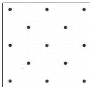
Pattern 5 Hole spacing: 12.0mm x 6.0mm Hole size: 1.1 ± 0.2mm
