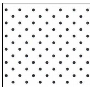
Pattern 3 Hole spacing: 5.0mm x 2.5mm Hole size: 1.2 ± 0.2mm
