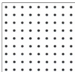
Pattern 2 Hole spacing: 3.5mm x 0.0mm Hole size: 1.1 ± 0.2mm
