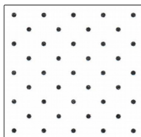
Pattern 1 Hole spacing: 7.0mm x 3.5mm Hole size: 1.1 ± 0.2mm
